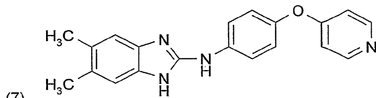
(5,6-Dimethyl-1H-benzimidazol-2-yl)-[4-(pyridin-4-yloxy)-phenyl]-amin
